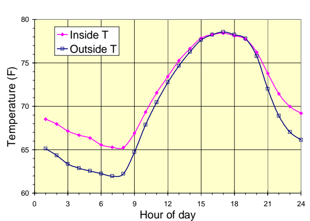
Figure 2. Average hourly air temperatures within each of the study barns for August 2000.
